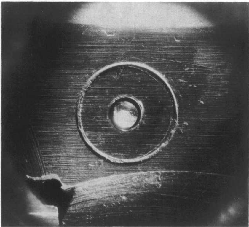
BREECH FACE AND FIRING PIN - C15
