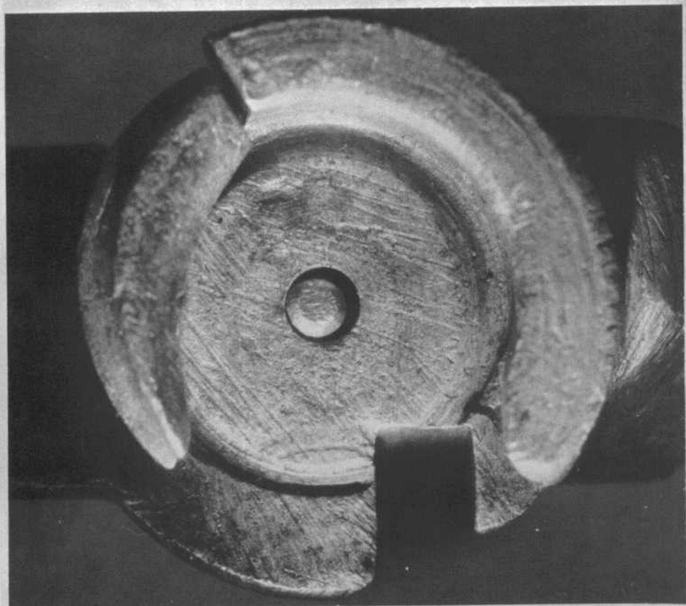
FACE OF BOLT OF CI4 RIFLE
